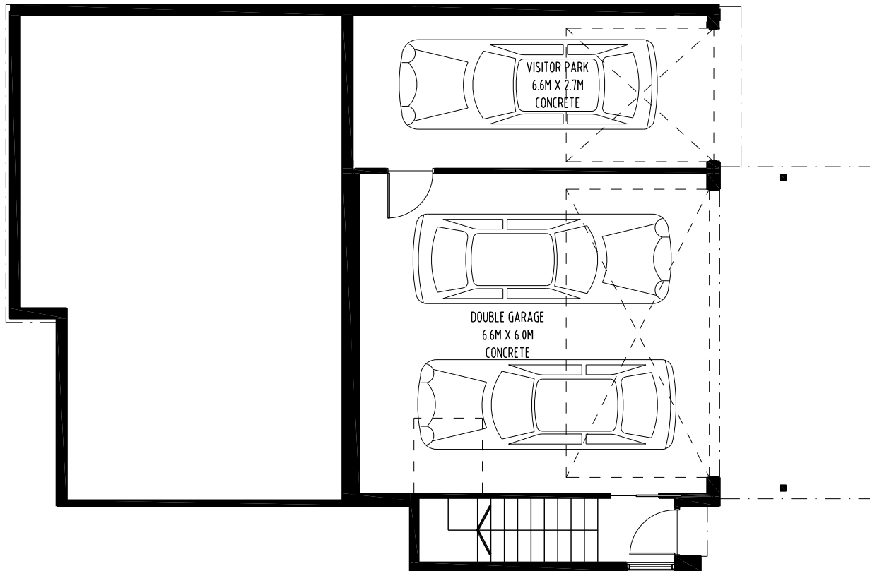
01 TOWN HOUSE 3 - LEVEL 1 PLAN - 1:100
