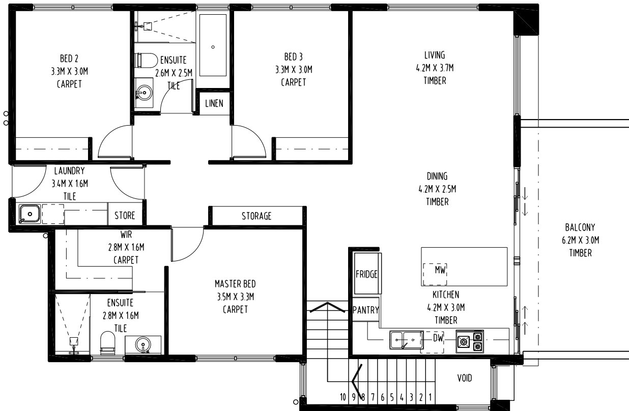
01 TOWN HOUSE 3 - LEVEL 2 PLAN - 1:100
