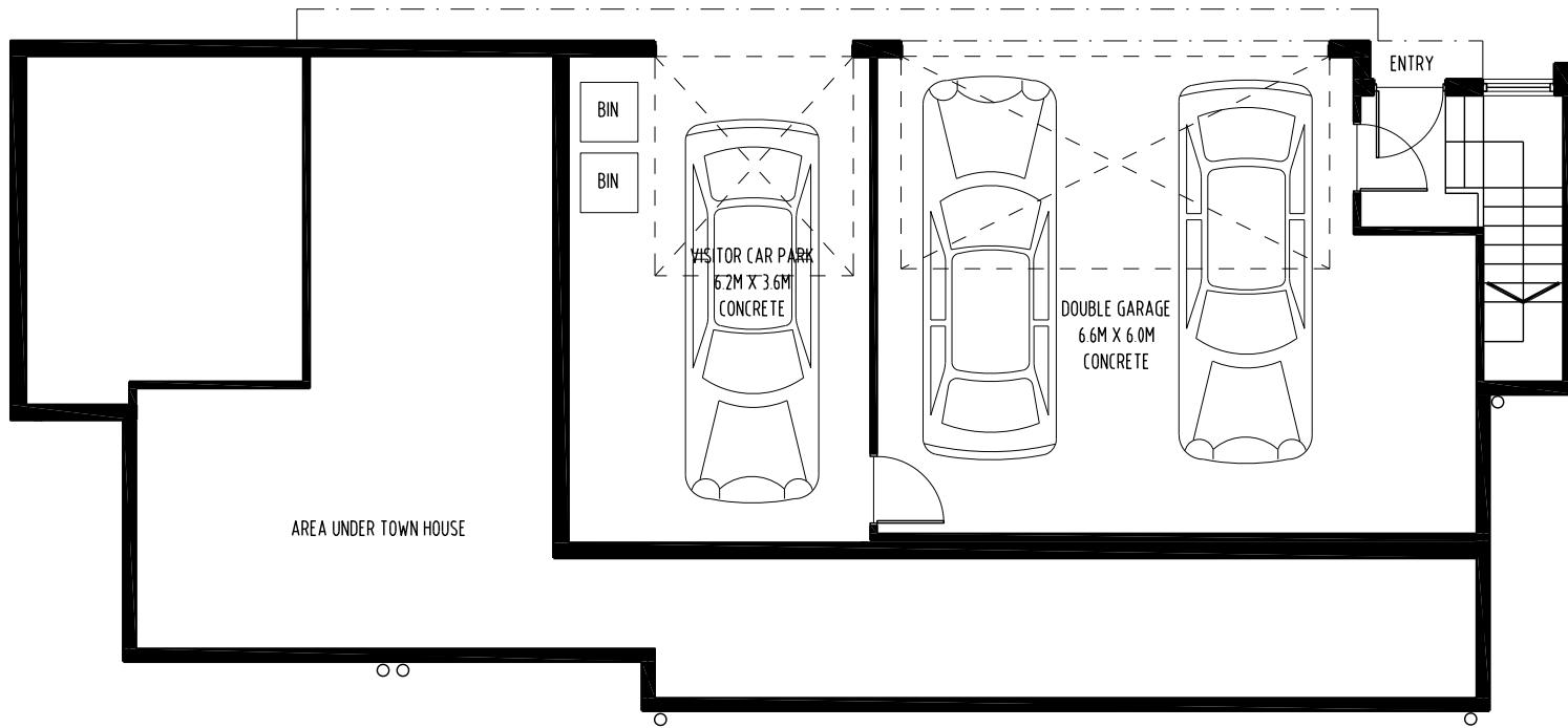
01 TOWN HOUSE 1 - LEVEL 1 PLAN - 1:100
